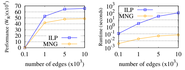
Figure 6: Results on synthetic datasets. (a) Performance as weight of recommendation ( W_R ) of ILP and MNG. (b) Runtime of ILP and MNG (seconds).
