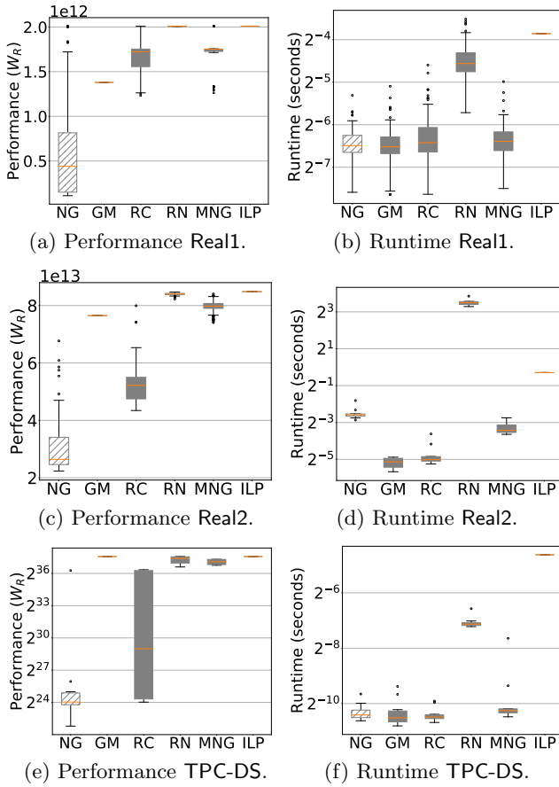
Figure 5: Performance and runtime of methods on real datasets. No clear winner.
