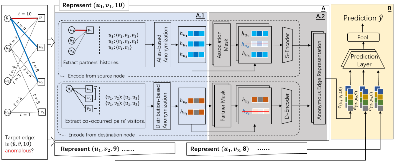
Figure 1: Illustration of the anomaly detection framework AER-AD. (A) Representation Module; (A.1) Edge Anonymization module; (A.2) Representation Learning Module; (B) Prediction Module.
