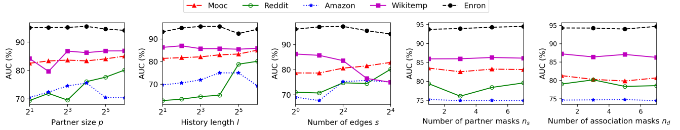
Figure 4: Varying hyper-parameters.
