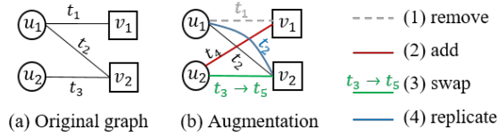
Figure 3: Data augmentation
